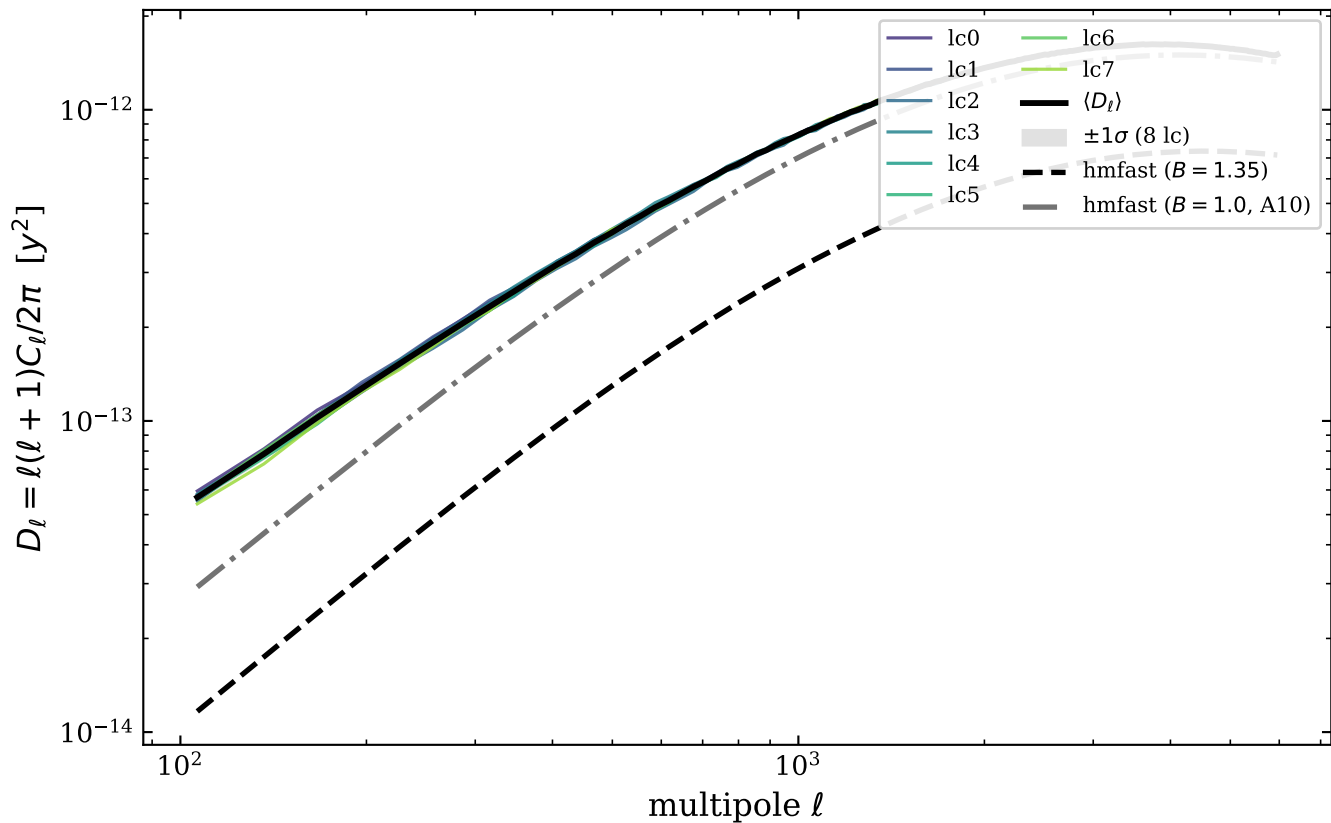
L2p8_m9 masked tSZ PS — q > 10
