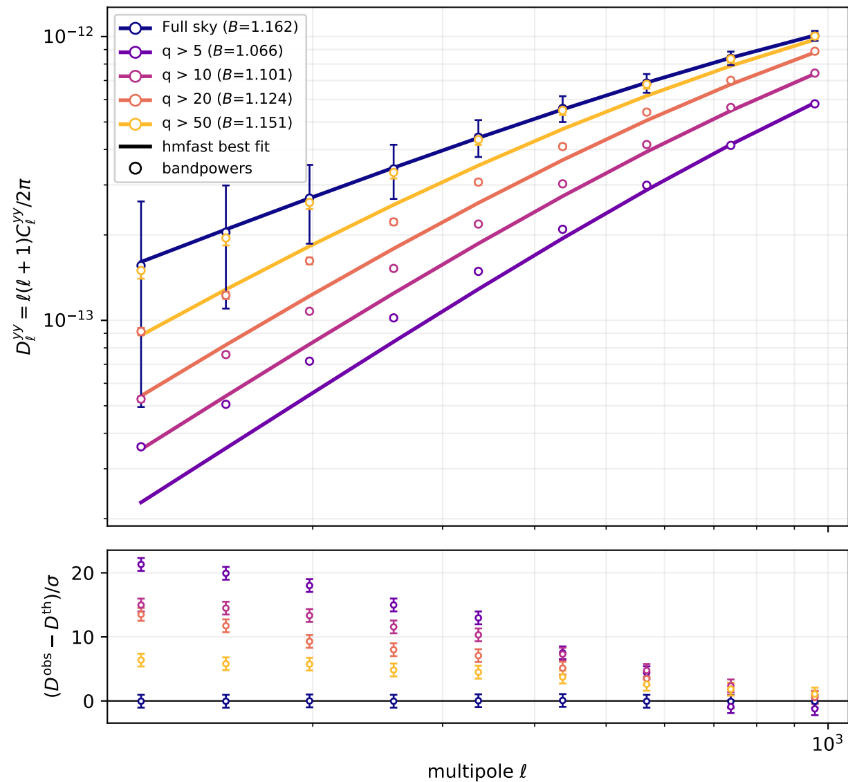
Best-fit tSZ PS (arnaudB1, \ell > 100 ; A10 GNFW, \sigma_{\ln \gamma} = 0.173 )
