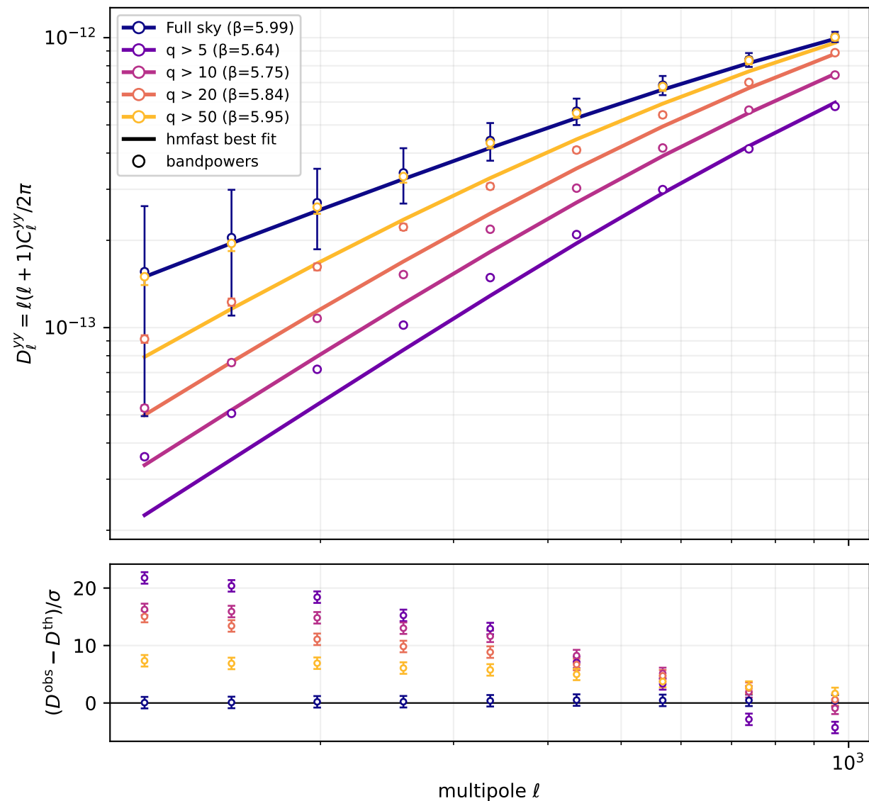
Best-fit tSZ PS, vary \beta (arnaudB1, \ell > 100 ; B = 1 , \sigma_{\ln Y} = 0.173 )
