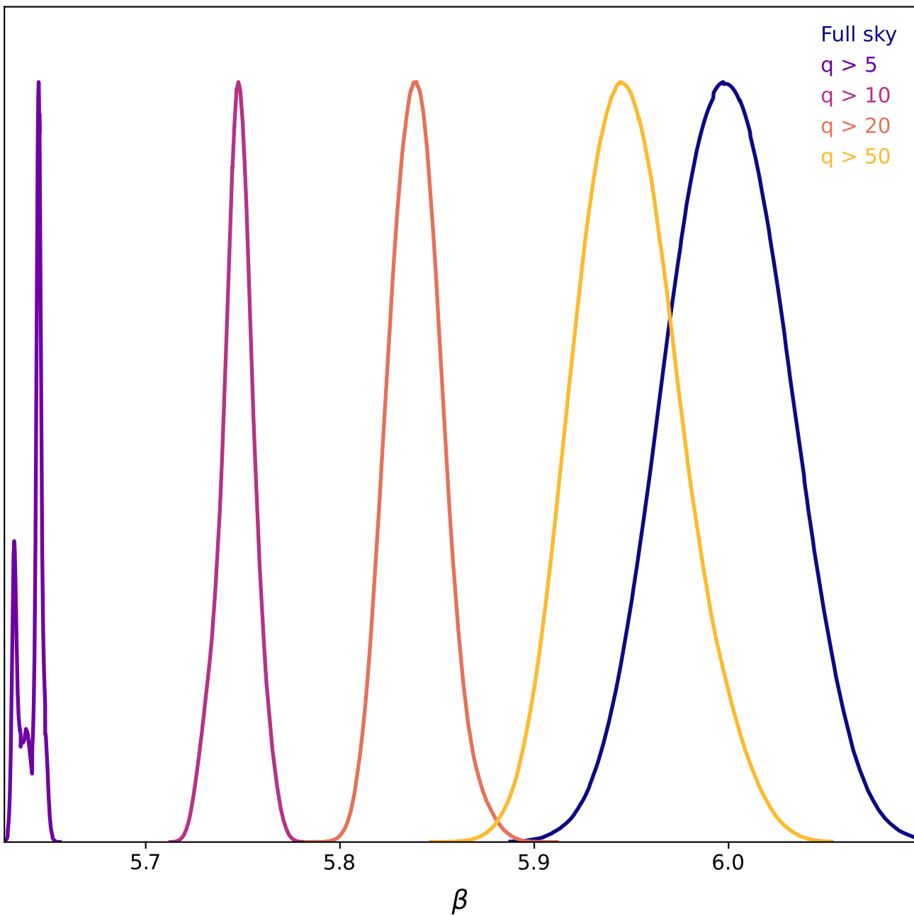
Posterior of GNFW outer slope \beta (arnaudB1, \ell > 100 , B = 1 , \sigma_{\ln \gamma} = 0.173 )
