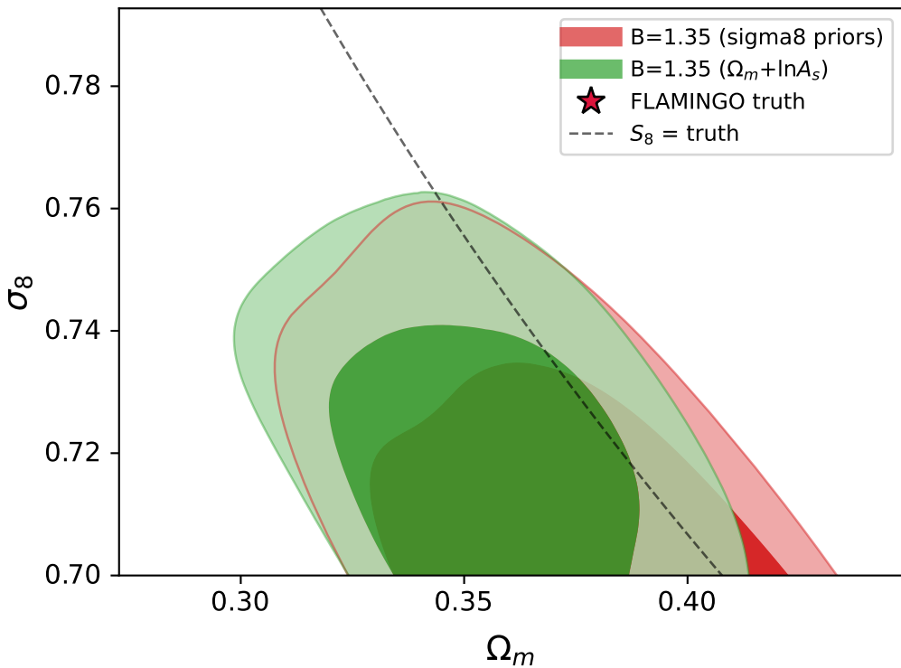
B=1.35: sigma8 vs \Omega_m + \ln A_s priors
