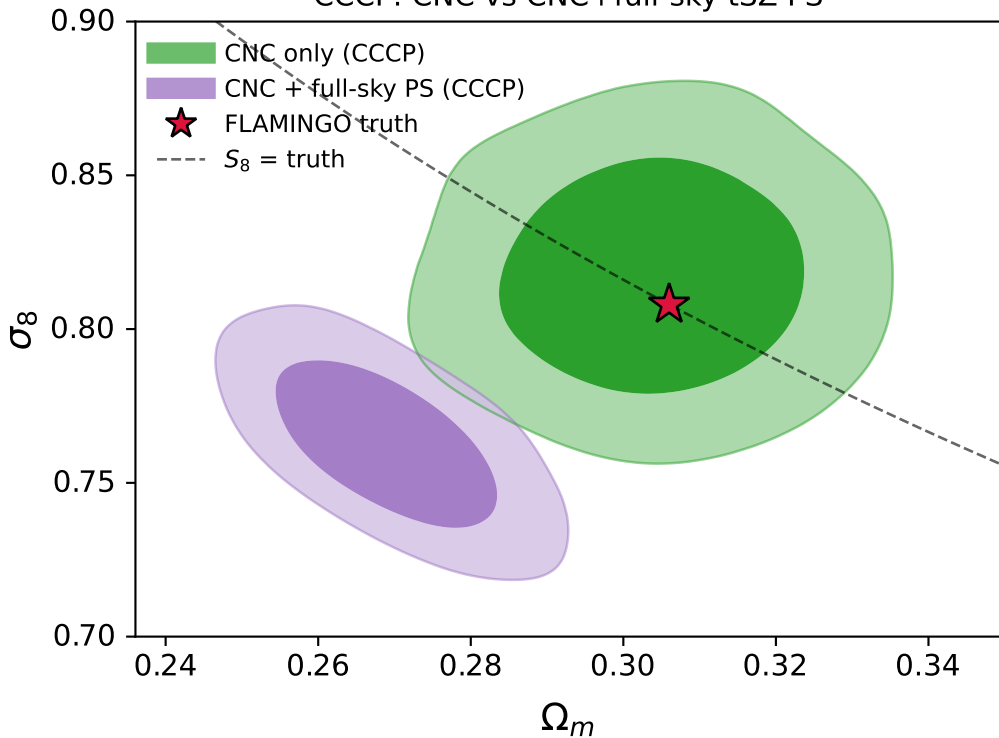
CCCP: CNC vs CNC+full-sky tSZ PS
