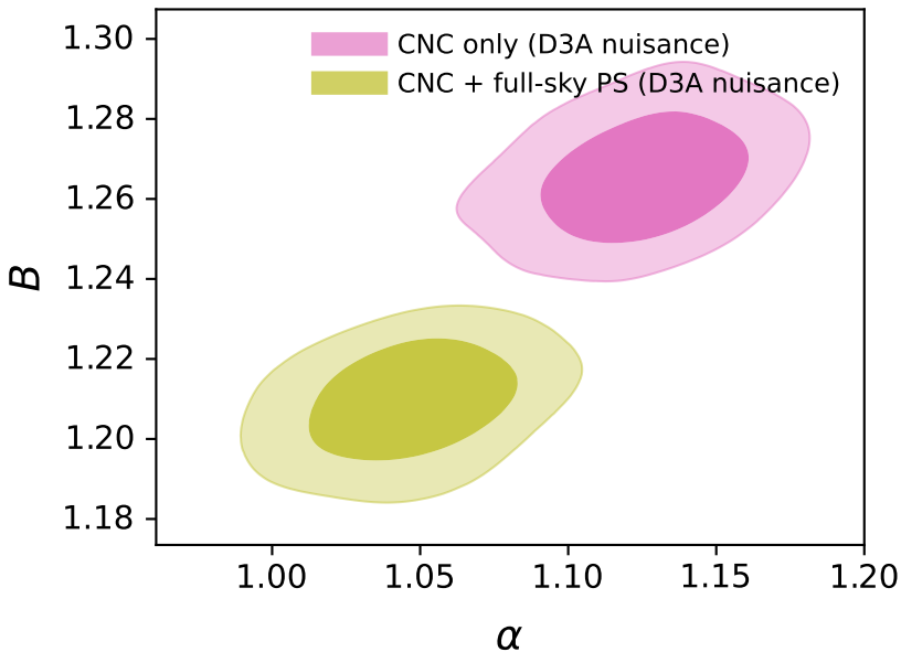
D3A nuisance: alpha_SZ vs B
