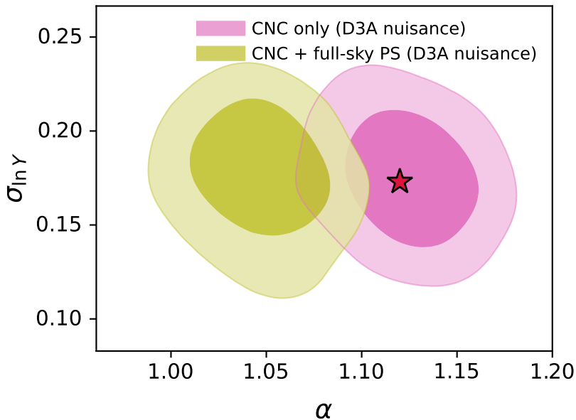
D3A nuisance: alpha_SZ vs sigma_InY
