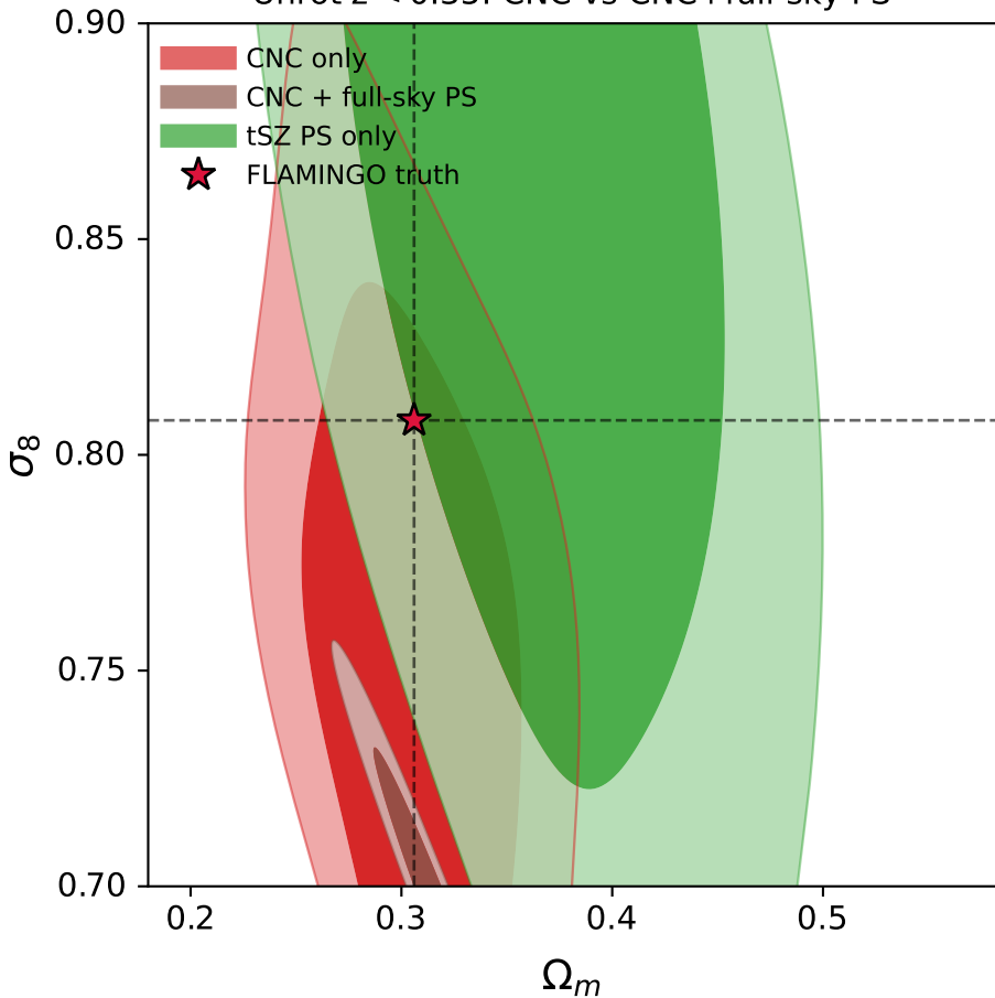
Unrot z < 0.35 : CNC vs CNC+full-sky PS
