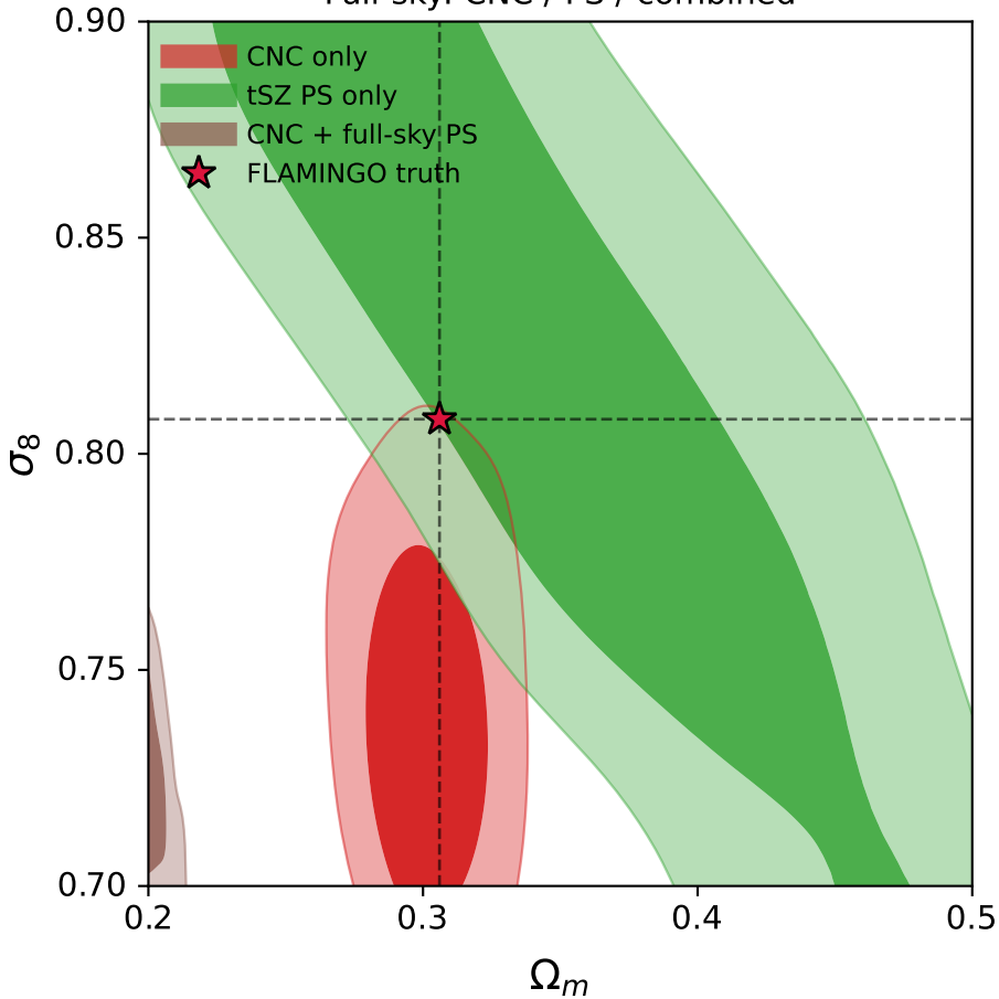
Full-sky: CNC / PS / combined
