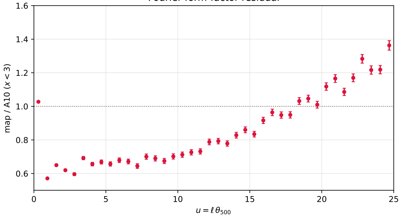
Fourier form-factor residual
