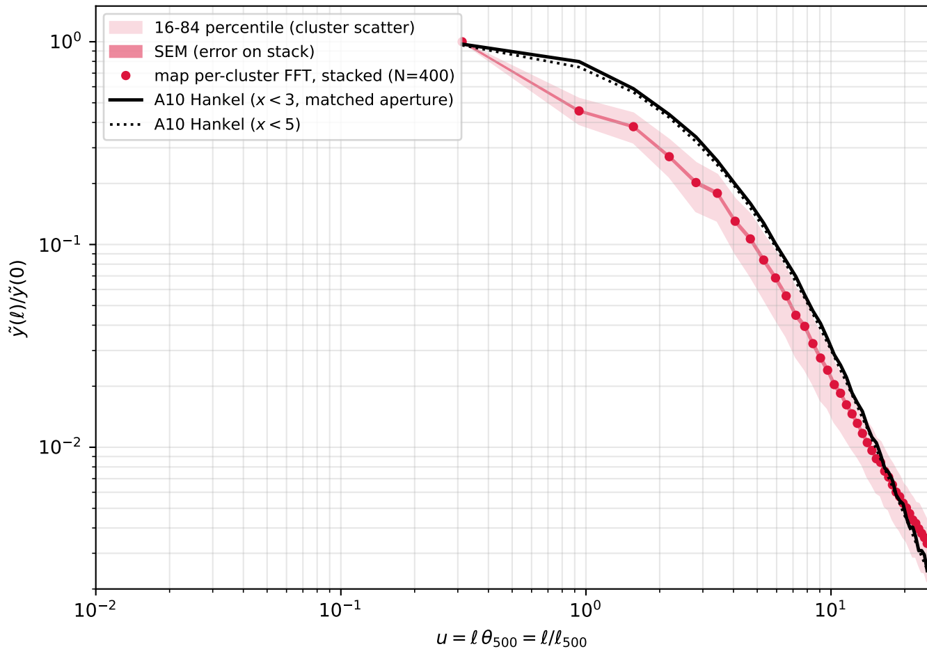
Fourier-space stacked tSZ profile vs Arnaud A10
