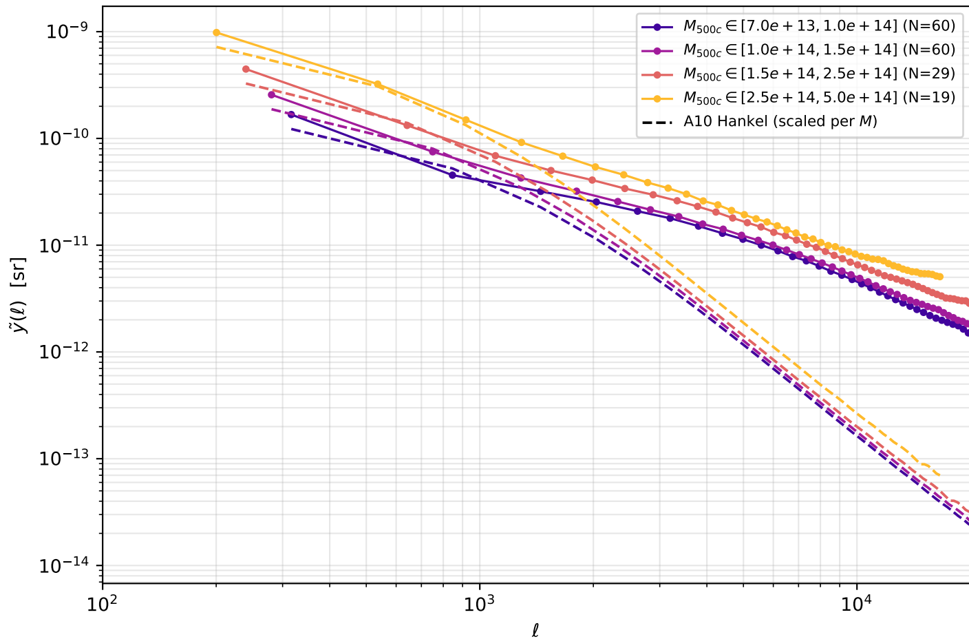
Raw \tilde{y}(\ell) vs mass at fixed z ( z \in [0.04, 0.05] , \bar{z} = 0.046 )
