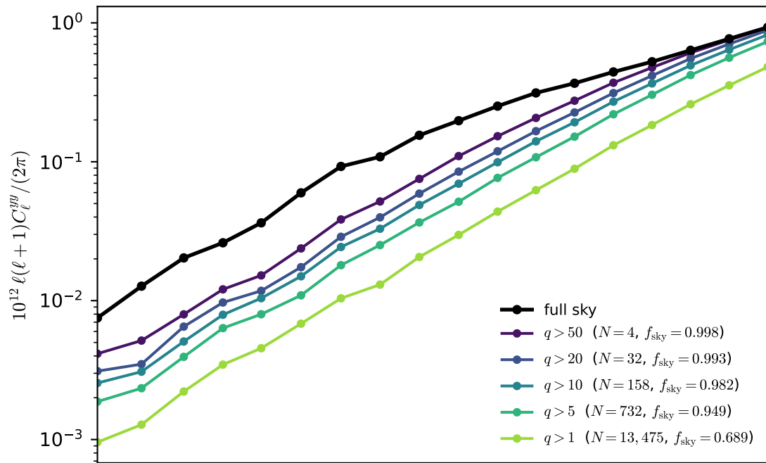
FLAMINGO L1_m9 fiducial: masked tSZ power spectrum ( \alpha_{\text{SZ}} = 1.12 best-fit q , 18 Planck bins)
