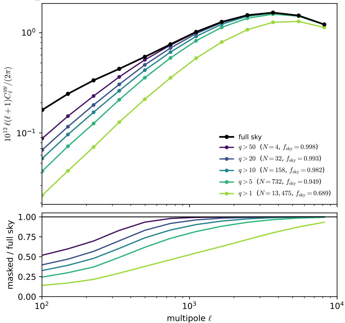
FLAMINGO L1_m9 fiducial: masked tSZ power spectrum ( \alpha_{\text{SZ}} = 1.12 best-fit q , \Delta \ln \ell = 0.4 log bins)
