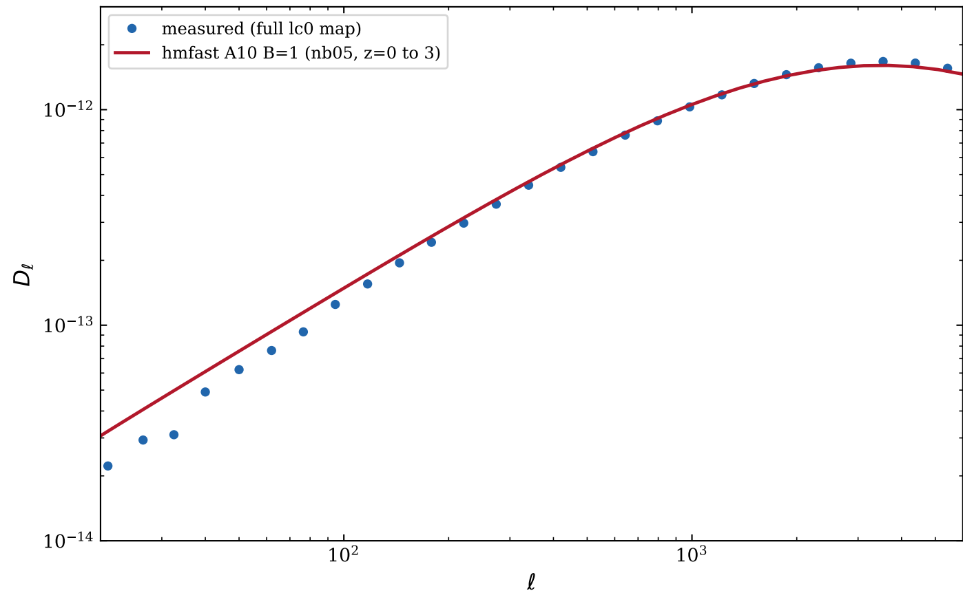
L2p8_m9 lc0: full-sky tSZ D_\ell ( 0 \leq z < 3 )
