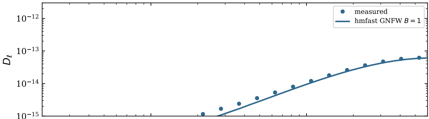
shell 18 z \in [0.900, 0.950] ( z_{\text{mid}} \approx 0.93 ) — snap59 ( z=0.95 ), snap60 ( z=0.90 )
