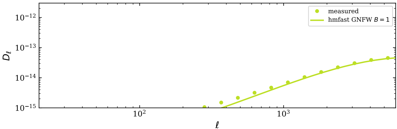
shell 21 z \in [1.050, 1.100] ( z_{\text{mid}} \approx 1.08 ) — snap56 ( z=1.10 ), snap57 ( z=1.05 )
