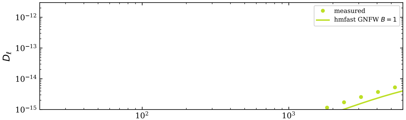
shell 41 z \in [2.050, 2.100] ( z_{\text{mid}} \approx 2.08 ) — snap36 ( z=2.10 ), snap37 ( z=2.05 )
