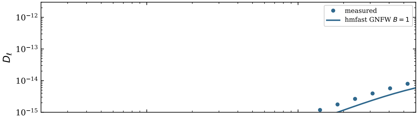
shell 38 z \in [1.900, 1.950] ( z_{\text{mid}} \approx 1.92 ) — snap39 ( z=1.95 ), snap40 ( z=1.90 )
