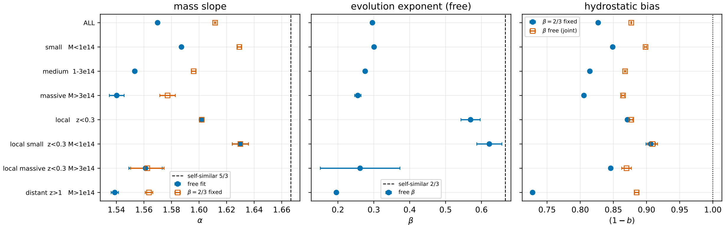
Subsample fits: mass slope, evolution, and bias under different fixings (fitted-alpha (1-b); error bars = OLS SE)
