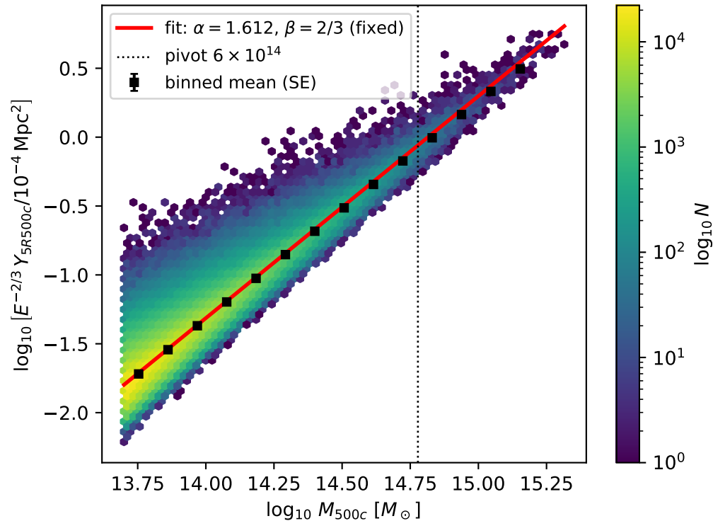
Y-M relation (self-similar E^{-2/3} removed)
