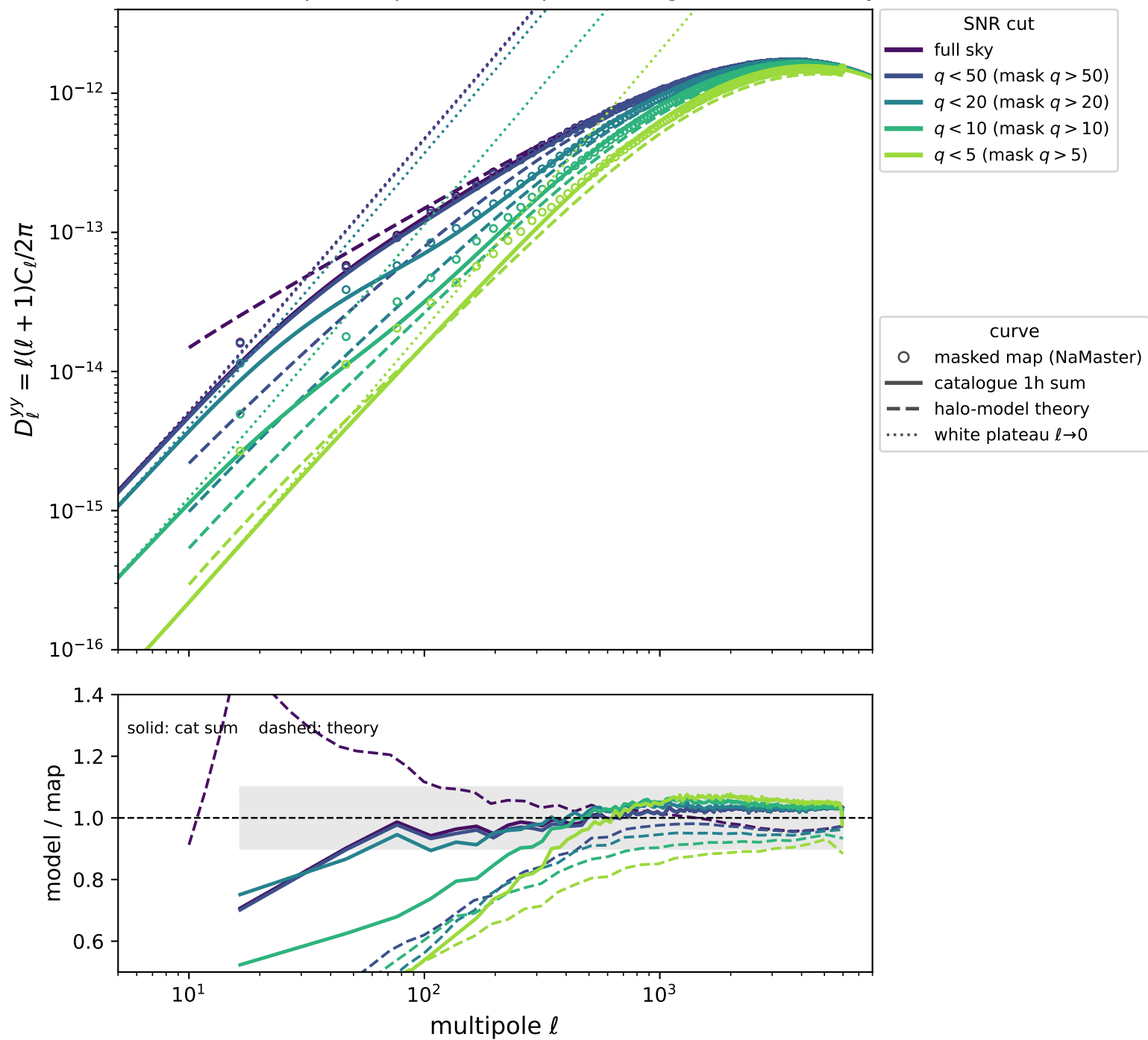
SNR-masked 1-halo tSZ power spectrum: map vs catalogue sum vs theory ( B = 1 )
