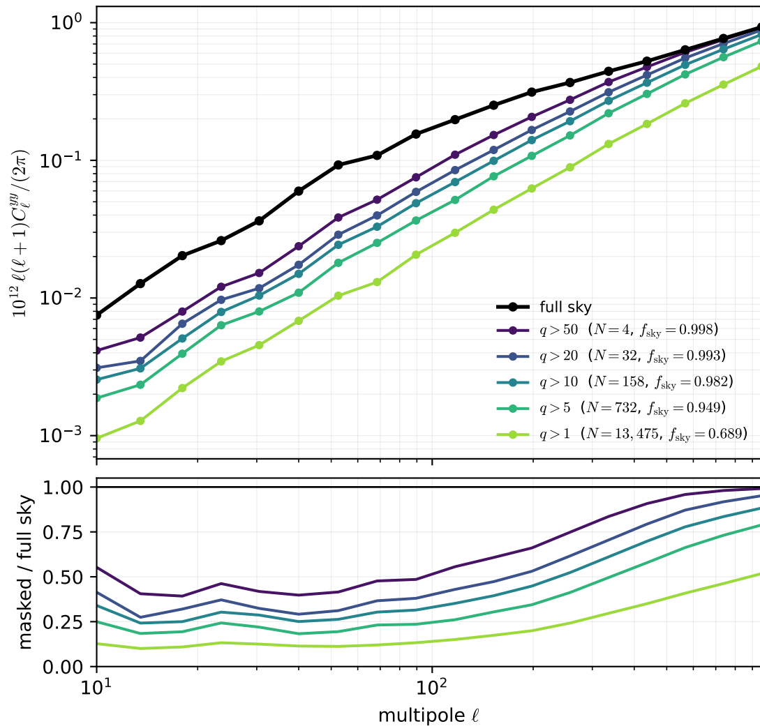
FLAMINGO L1_m9 fiducial: masked tSZ power spectrum ( \alpha_{\text{SZ}} = 1.12 best-fit q , 18 Planck bins)
