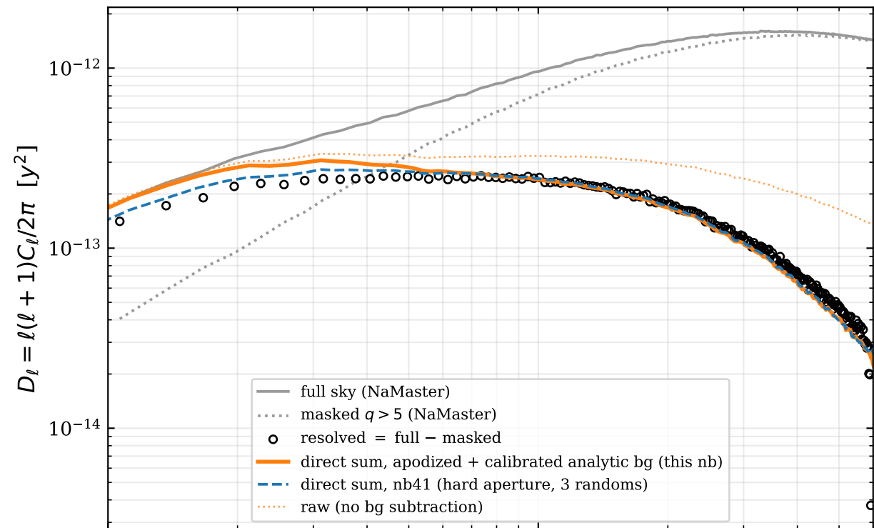
L1_m9 fiducial: resolved tSZ power ( q > 5 , 1088 clusters)
