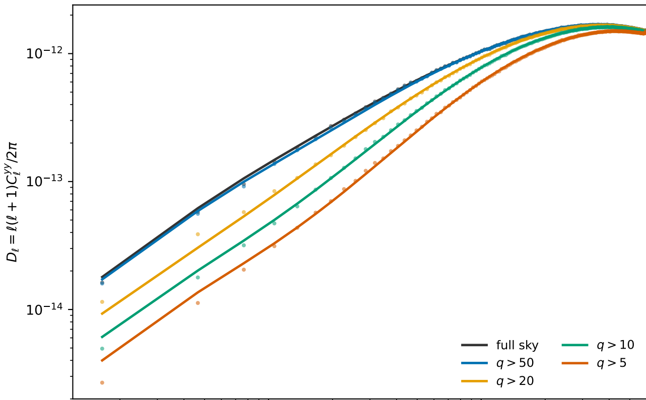
Universal catalogue-anchored tSZ model vs FLAMINGO
