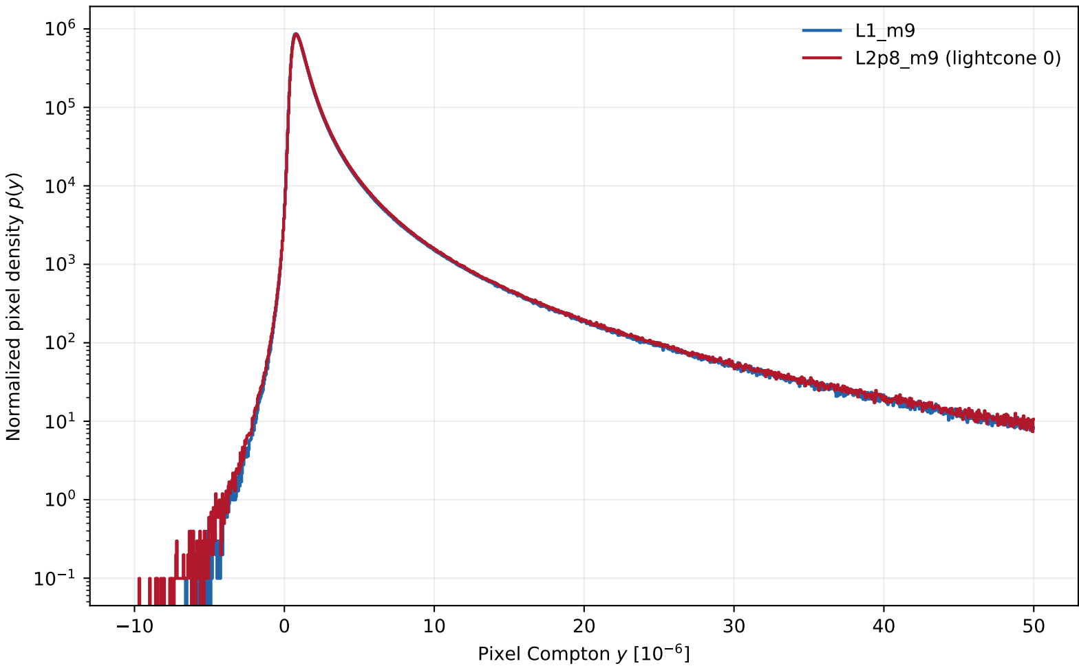
Fiducial Compton-y pixel histograms
