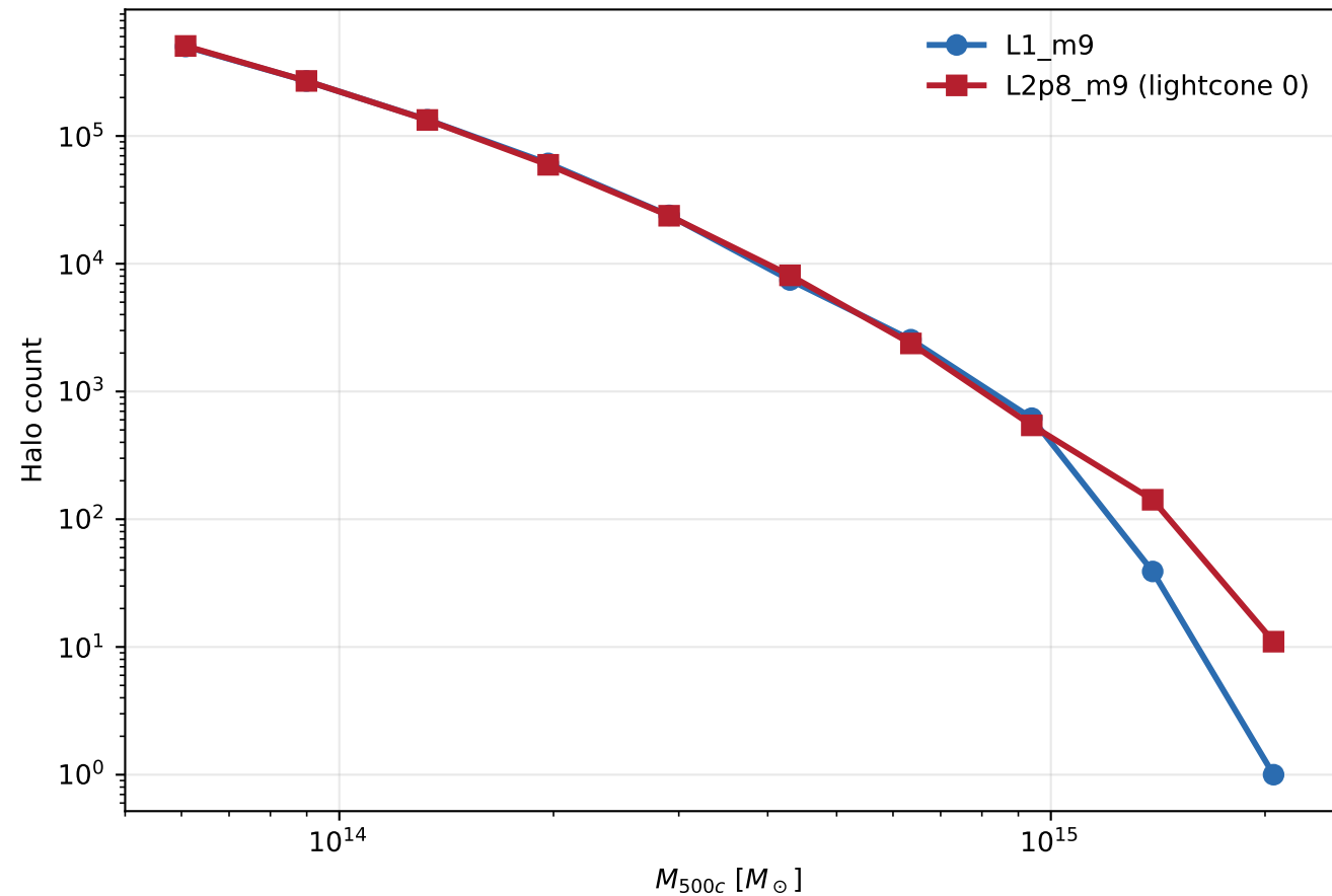
M_{500c} histogram ( 0.005 \leq z \leq 1 )
