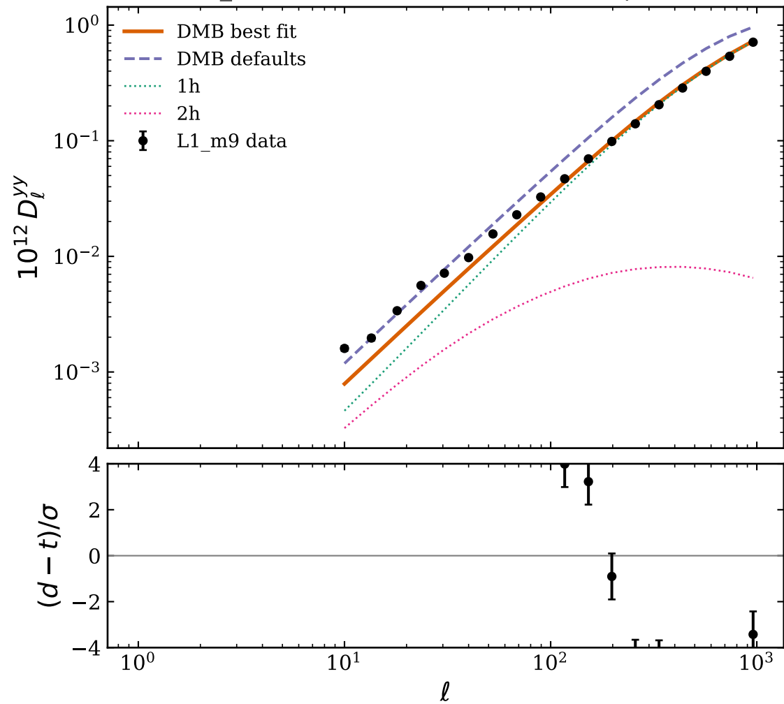
L1_m9 masked tSZ PS — DMB fit ( q > 10 )
