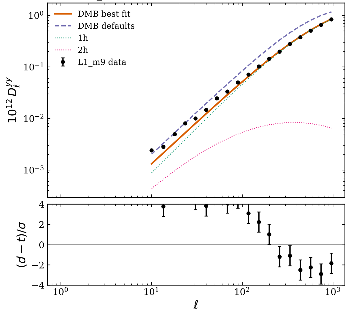
L1_m9 masked tSZ PS — DMB fit ( q > 20 )
