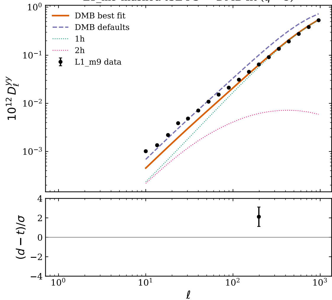
L1_m9 masked tSZ PS — DMB fit ( q > 5 )
