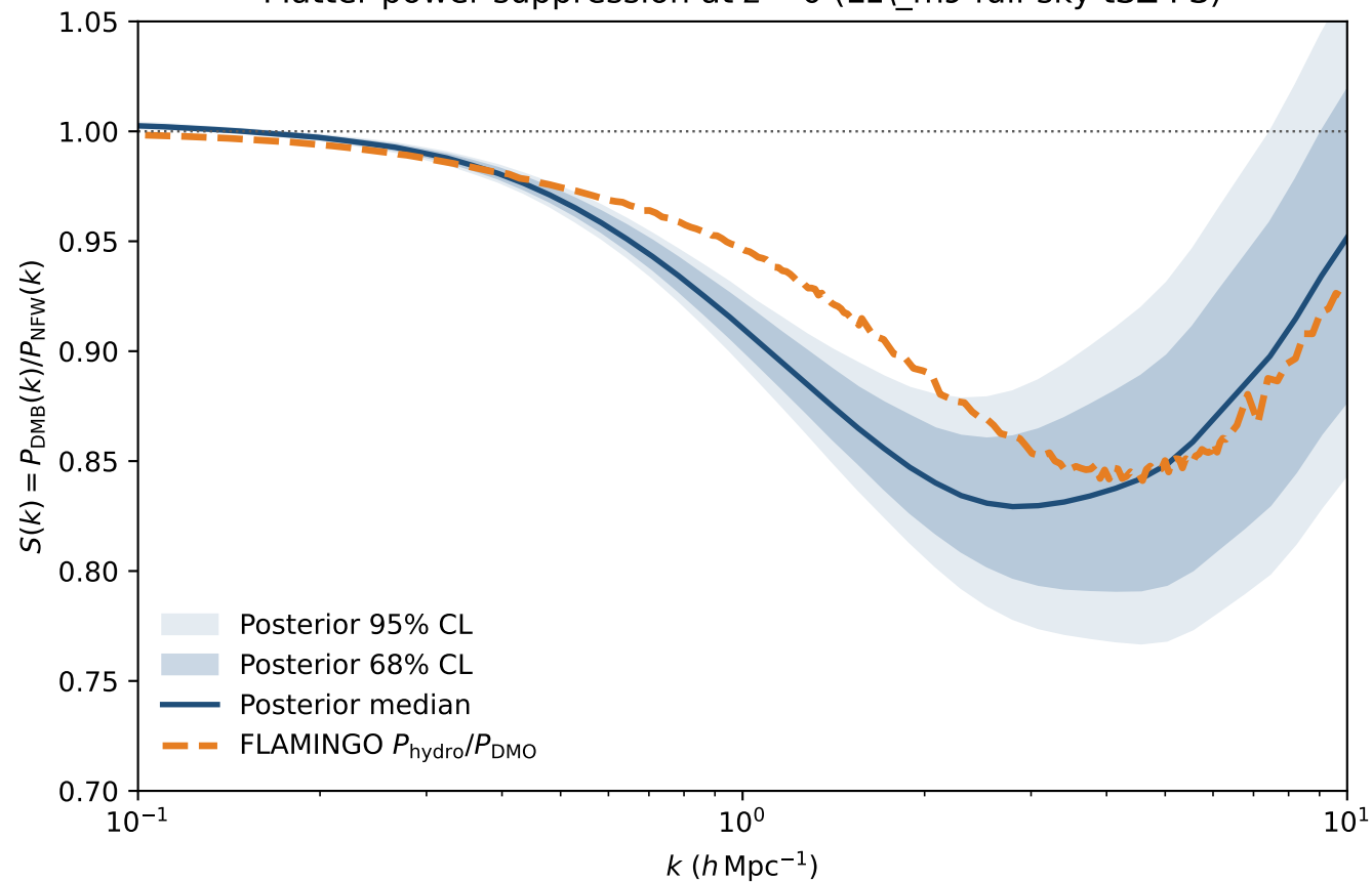
Matter power suppression at z = 0 (L1\_m9 full-sky tSZ PS)
