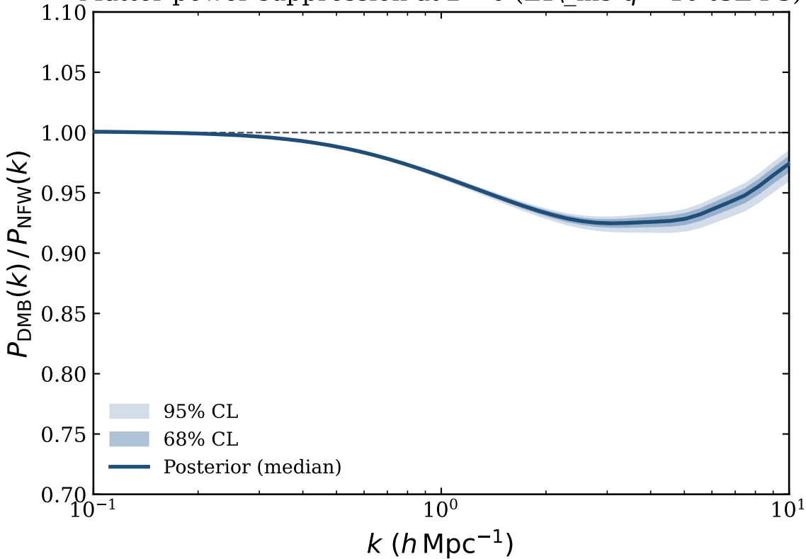
Matter power suppression at z = 0 (L1\_m9 q > 10 tSZ PS)
