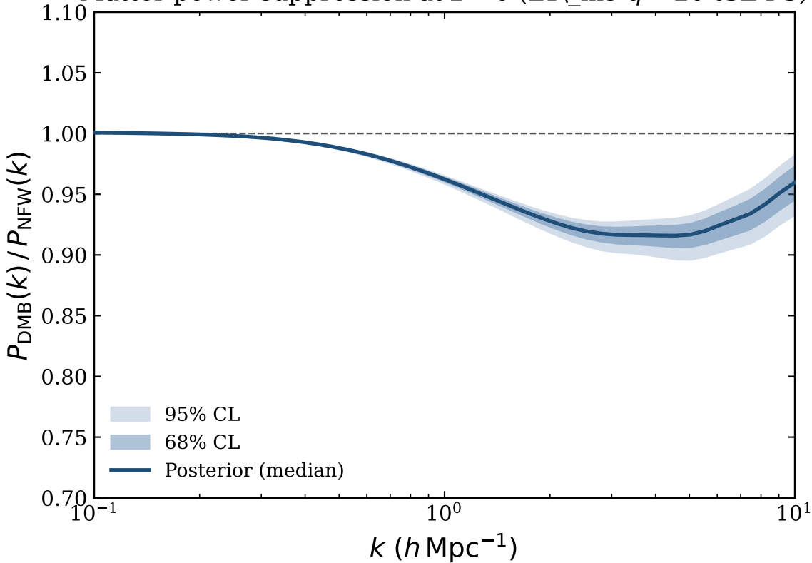
Matter power suppression at z = 0 (L1\_m9 q > 20 tSZ PS)
