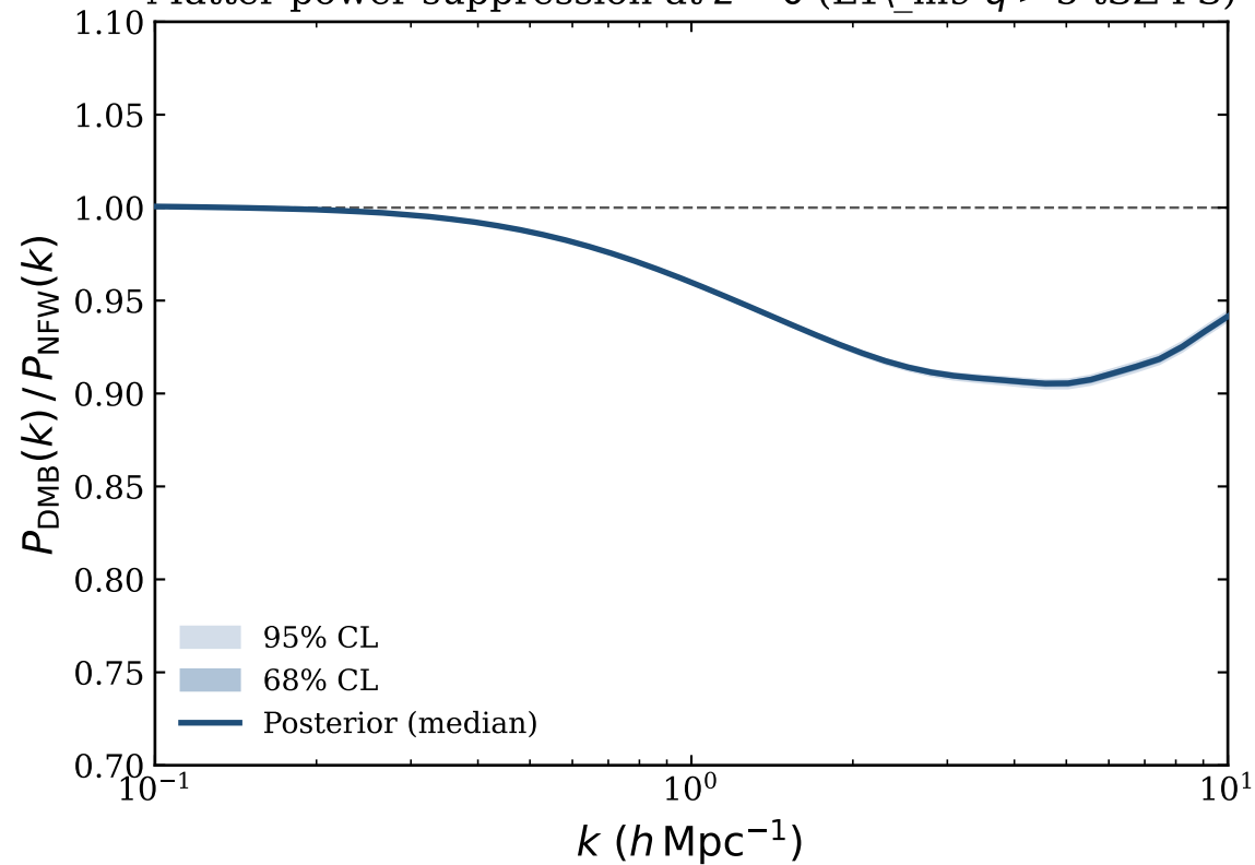
Matter power suppression at z = 0 (L1\_m9 q > 5 tSZ PS)
