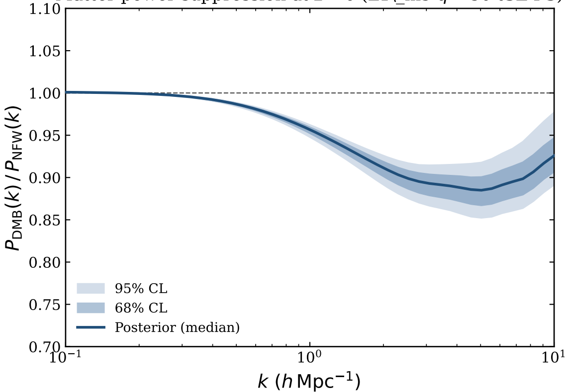
Matter power suppression at z = 0 (L1\_m9 q > 50 tSZ PS)
