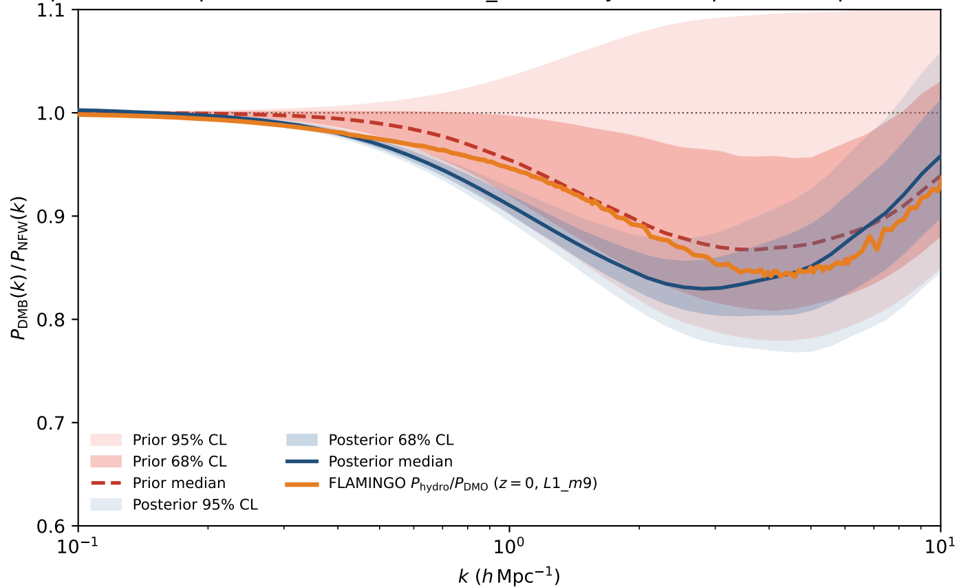
Prior predictive vs posterior S(k) at z = 0 (L1\_m9 full-sky tSZ PS; prior=500, post=128 draws)
