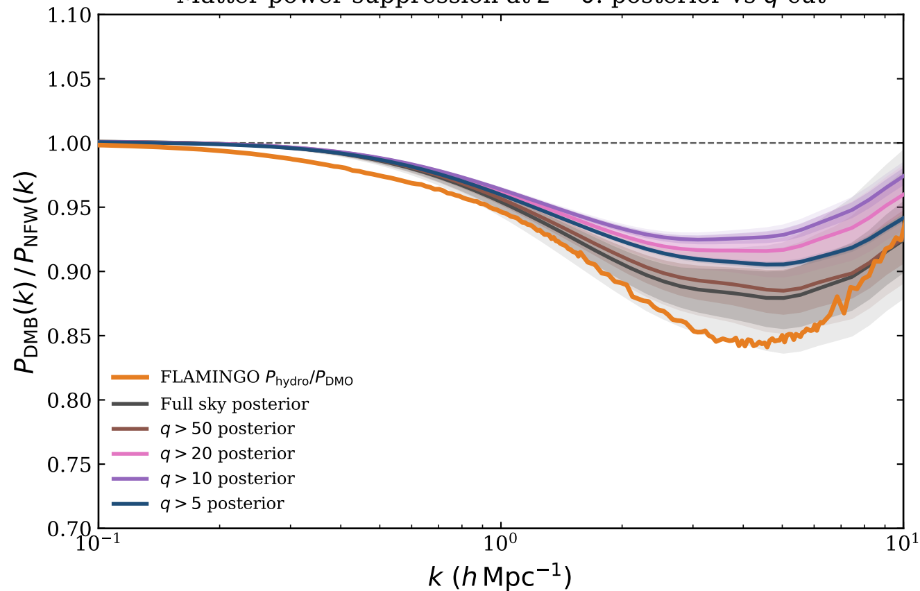
Matter power suppression at z = 0 : posterior vs q -cut
