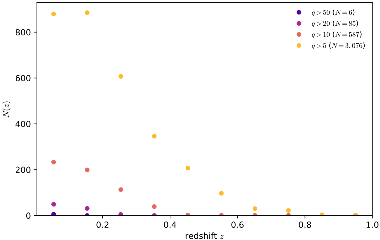
FLAMINGO L1_m9 binned CNC: N(z) vs detection cut (10 linear z bins, 5 log q bins ( q_{\text{cut}} to 8q_{\text{cut}} ); empirical aperture q )
