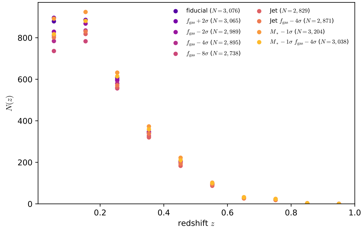
FLAMINGO L1_m9 binned CNC: N(z) at q > 5 by feedback (10 linear z bins, 5 log q bins ( q_{\text{cut}} to 8q_{\text{cut}} ); empirical aperture q )
