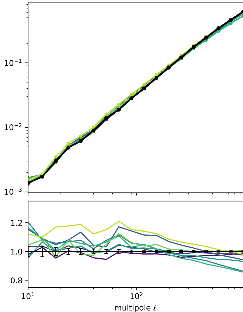
FLAMINGO L1_m9 feedback variants: tSZ power spectrum (18 Planck bins; q from \alpha_{SZ} = 1.12 best fit) errors: custom-GNFW \alpha_{SZ} = 1.12 , B = 1.41 , best-fit A_{SZ} covariance full sky masked, q > 5
