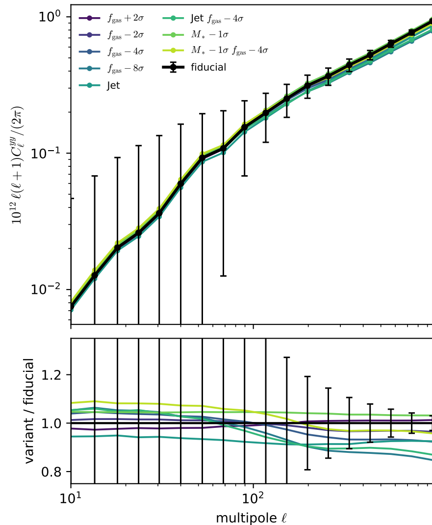
FLAMINGO L1_m9 feedback variants: tSZ power spectrum (18 Planck bins; q from \alpha_{SZ} = 1.12 best fit) errors: custom-GNFW \alpha_{SZ} = 1.12 , B = 1.41 , best-fit A_{SZ} covariance full sky masked, q > 5
