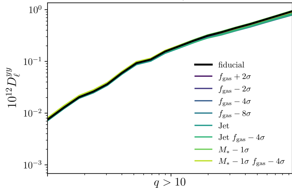
full sky
