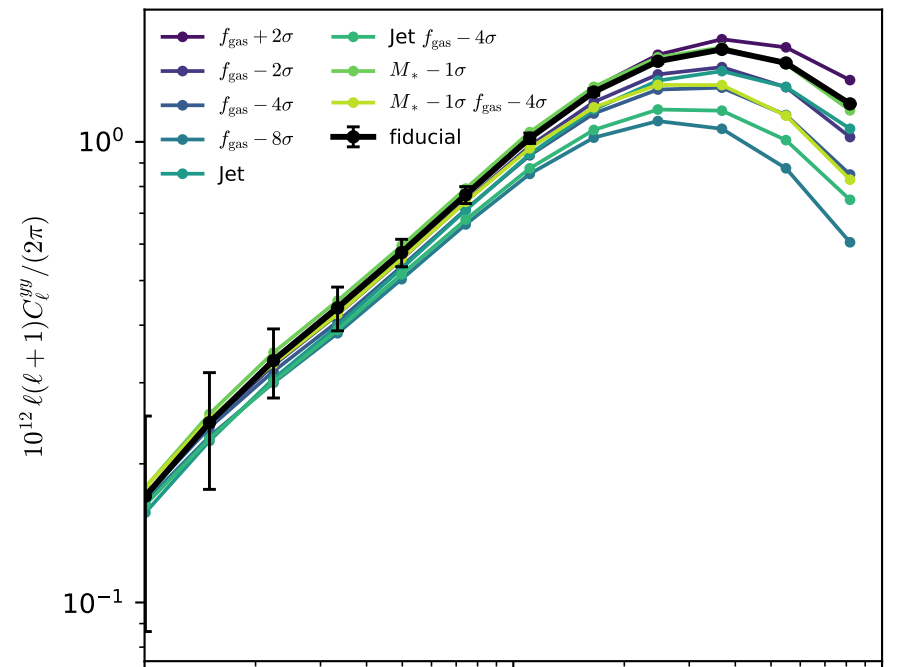
FLAMINGO L1_m9 feedback variants: tSZ power spectrum ( \Delta \ln \ell = 0.4 log bins; q from \alpha_{\text{SZ}} = 1.12 best fit)
