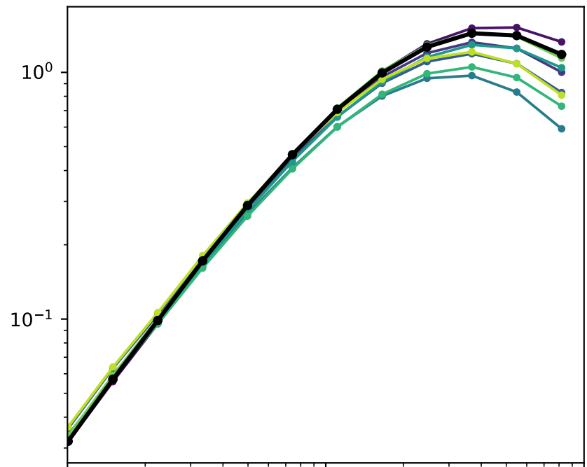
FLAMINGO L1_m9 feedback variants: tSZ power spectrum ( \Delta \ln \ell = 0.4 log bins; q from \alpha_{\text{SZ}} = 1.12 best fit)
