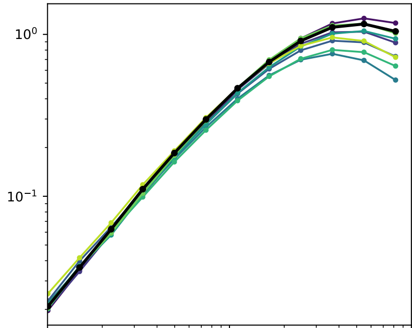
FLAMINGO L1_m9 feedback variants: tSZ power spectrum ( \Delta \ln \ell = 0.4 log bins; masked q > 1 ; q from \alpha_{\text{SZ}} = 1.12 best fit) errors: custom-GNFW \alpha_{\text{SZ}} = 1.12 , B = 1.41 , best-fit A_{\text{SZ}} covariance full sky masked, q > 1
