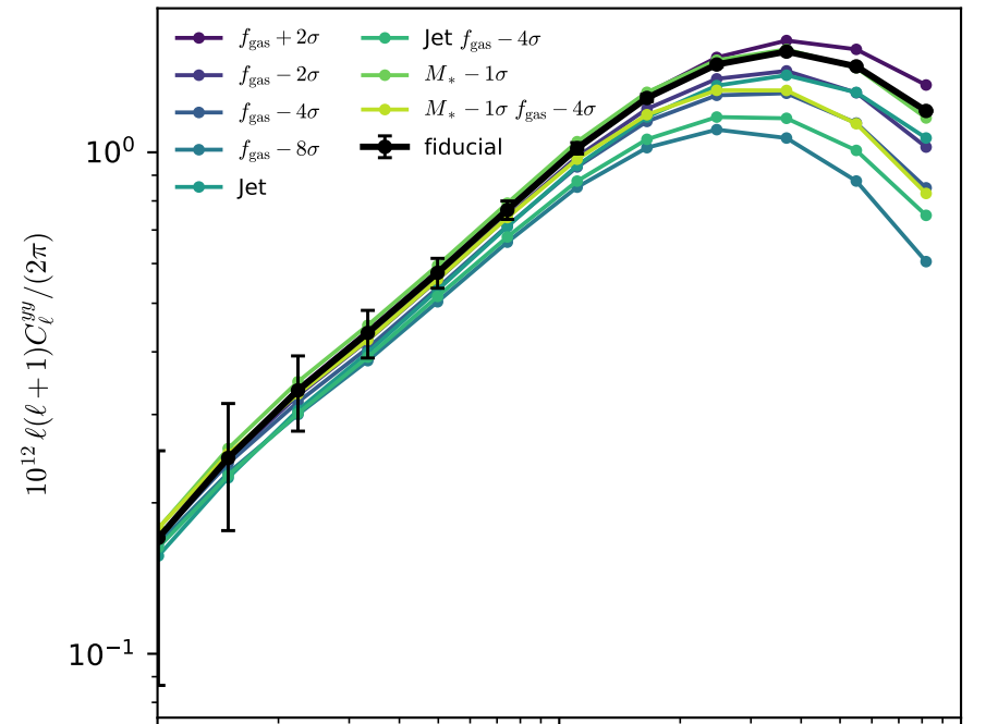
FLAMINGO L1_m9 feedback variants: tSZ power spectrum ( \Delta \ln \ell = 0.4 log bins; masked q > 1 ; q from \alpha_{\text{SZ}} = 1.12 best fit) errors: custom-GNFW \alpha_{\text{SZ}} = 1.12 , B = 1.41 , best-fit A_{\text{SZ}} covariance full sky masked, q > 1
