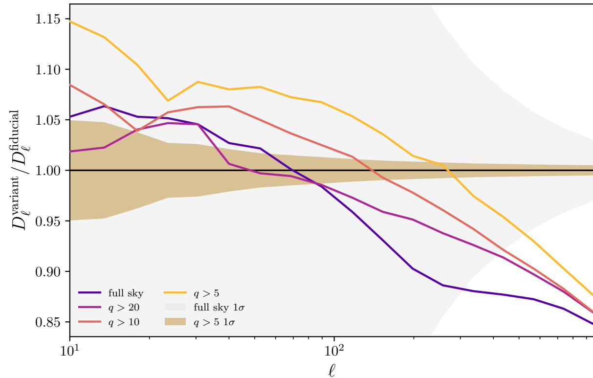
FLAMINGO L1_m9: f_{\text{gas}} - 8\sigma / fiducial ratio vs sky cut (18 Planck bins; empirical aperture q ; bands: full sky and q > 5 theory 1\sigma about 1)
