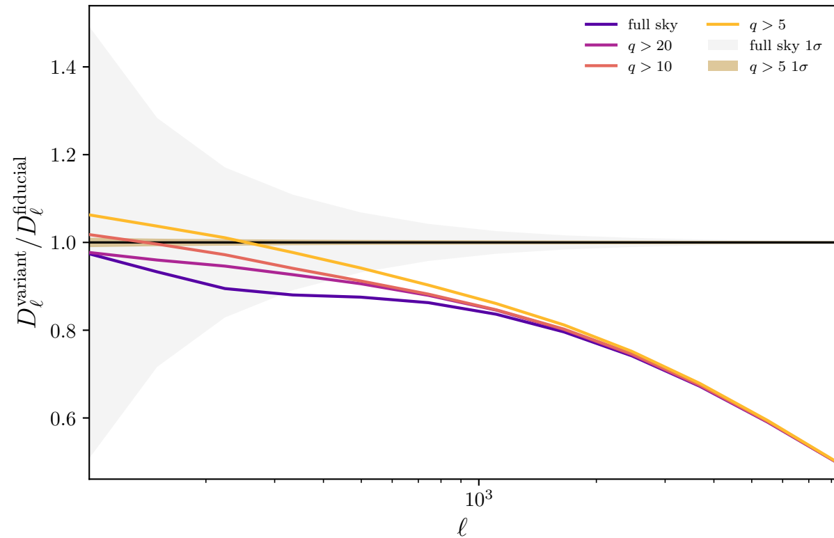
FLAMINGO L1_m9: f_{\text{gas}} - 8\sigma / fiducial ratio vs sky cut (12 log bins ( \Delta \ln \ell = 0.4 ); empirical aperture q ; bands: full sky and q > 5 theory 1\sigma about 1)
