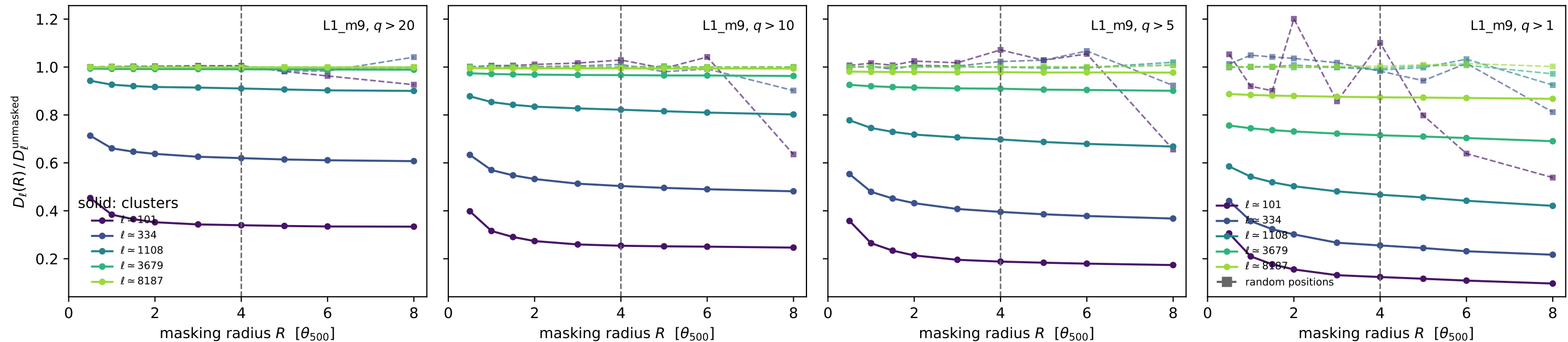
Masking-radius null test: random-position control
