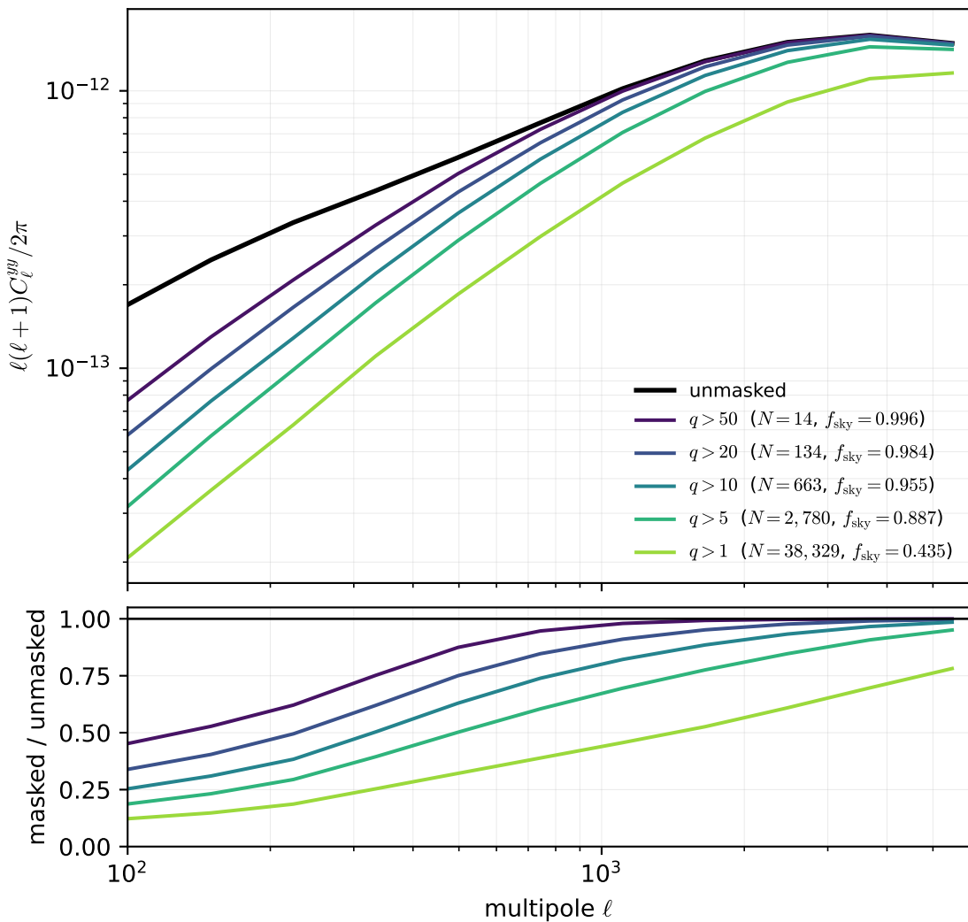
FLAMINGO L1_m9 fiducial: tSZ power spectrum masked at 4\theta_{500}
