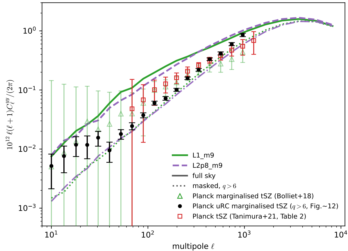
FLAMINGO fiducial tSZ vs Planck ( \alpha_{\text{SZ}} = 1.12 best-fit q )
