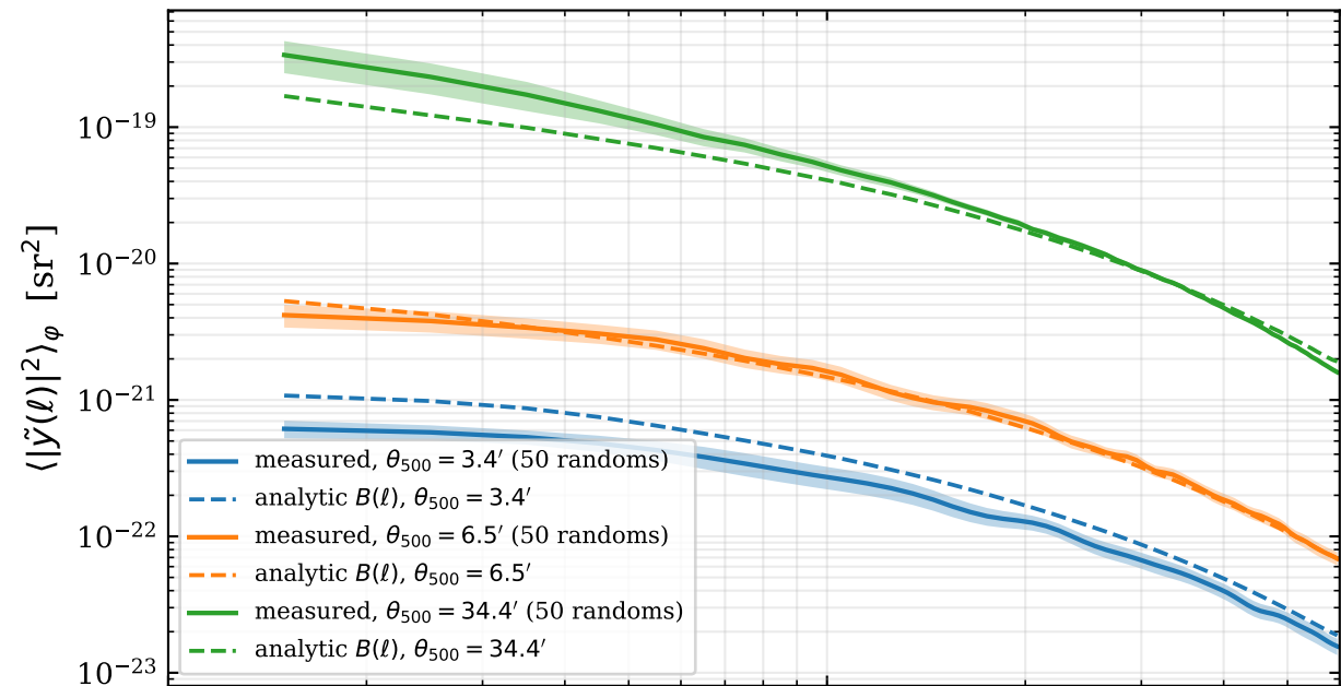
Random-aperture ensemble vs analytic background prediction
