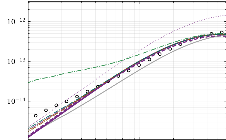
group 2: z \in [0.80, 1.35] , 3792 of 8,986,559 clusters
