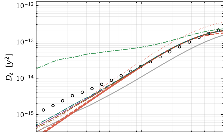
group 3: z \in [1.35, 2.20] , 3201 of 7,285,149 clusters
