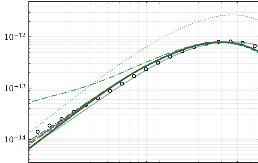
group 1: z \in [0.35, 0.80] , 4133 of 5,923,412 clusters
