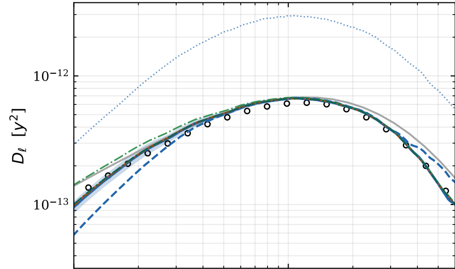
group 0: z \in [0.00, 0.35] , 4099 of 1,016,172 clusters
