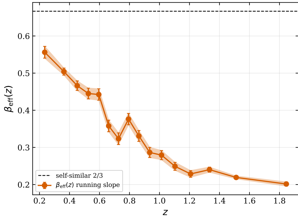
evolution exponent declines with z
