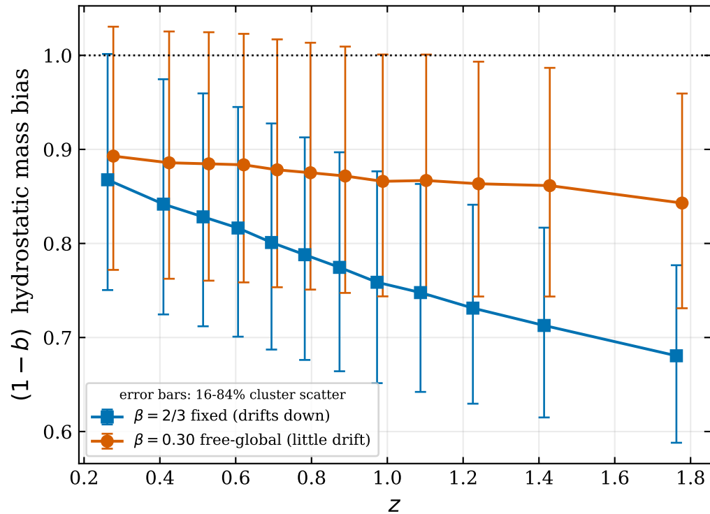
(1 - b) evolution depends on the \beta fixing
